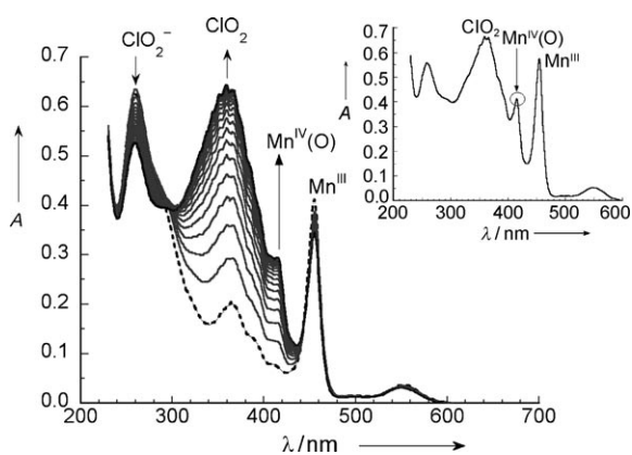
Figure 1. Repeat scan UV/Vis spectra for the dismutation of chlorite (4 mM) with [\text{Mn}(\text{TF}_4\text{TMAP})] (4 \mu\text{M} ) in phosphate buffer (pH 7.0 and \mu = 1.0\text{ M} ) at 25 °C. Spectra acquired every 8 min. The initial spectrum is black dashed line, ending spectrum in solid black, others in gray. Inset: reaction of 4.5 mM \text{ClO}_2^- with 8 \mu\text{M} [\text{Mn}(\text{TF}_4\text{TMAP})] after 100 min highlighting the observation of \text{Mn}^{\text{IV}}(\text{O}) at 417 nm.
