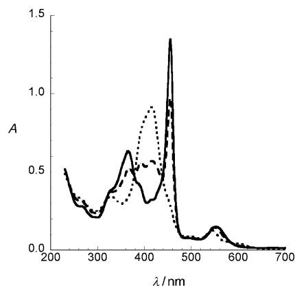
Figure 2. Spectral changes for the reaction of [\text{Mn}(\text{TF}_4\text{TMAP})] (14 \mu\text{M} ) and \text{ClO}_2^- (2 equiv) in borate buffer (pH 10.5 and \mu = 25\text{ mM} ) at 0 °C. Solid line is starting [\text{Mn}^{\text{III}}(\text{TF}_4\text{TMAP})] , dashed upon mixing, and dotted after 40 min. Final spectrum is that of \text{Mn}^{\text{IV}}(\text{O}) . [11]
